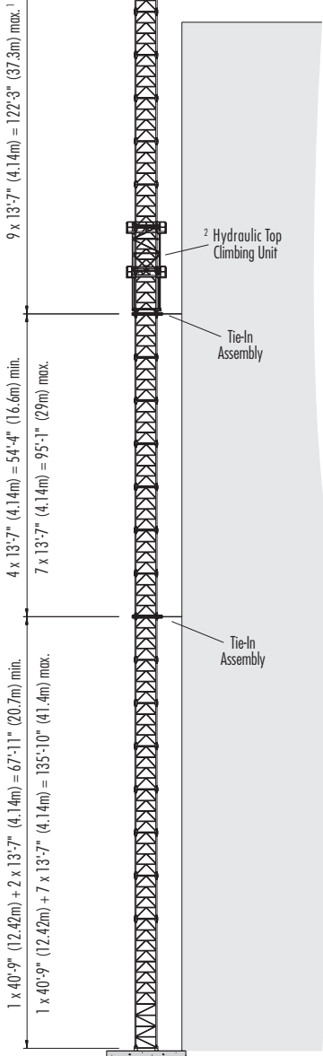
TOP CLIMBING with 290 HC Tower Sections tied to structure
